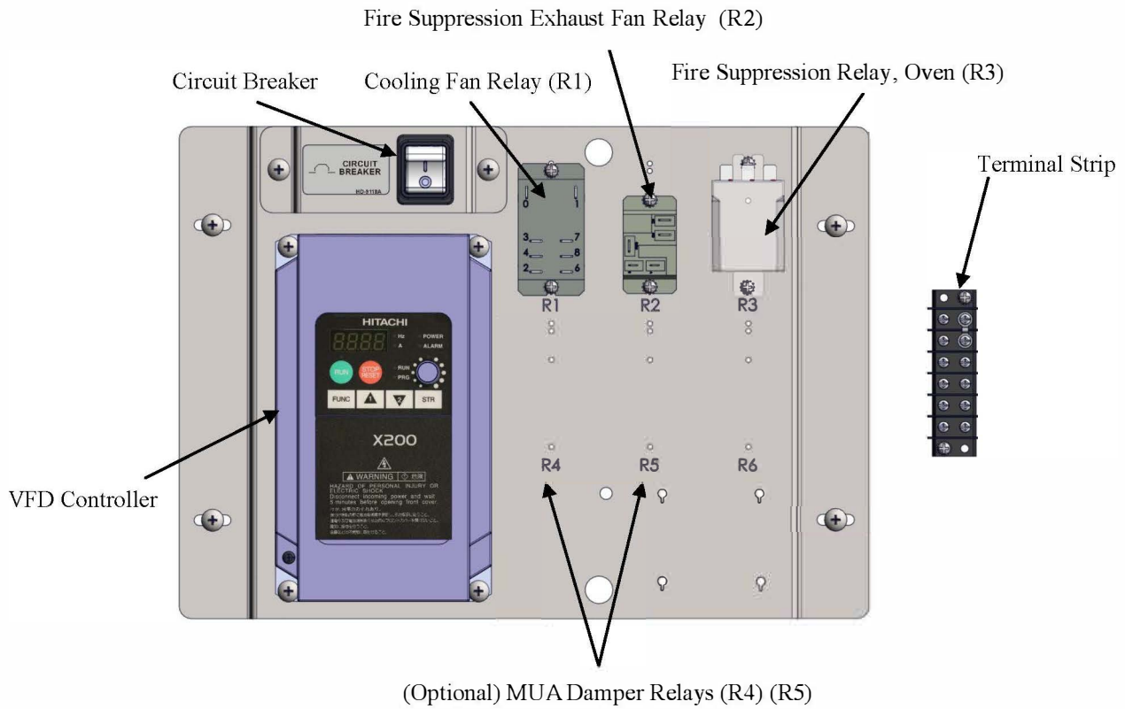
VFD Control Box (Cover removed)
