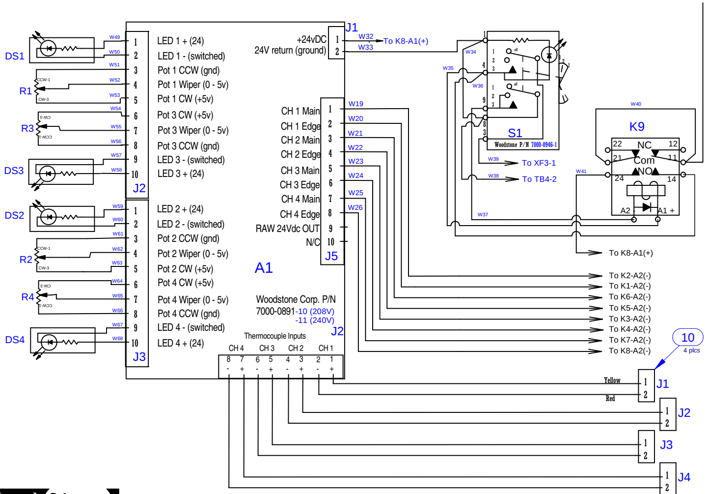
Low Voltage Controls and Power Latching Circuit
