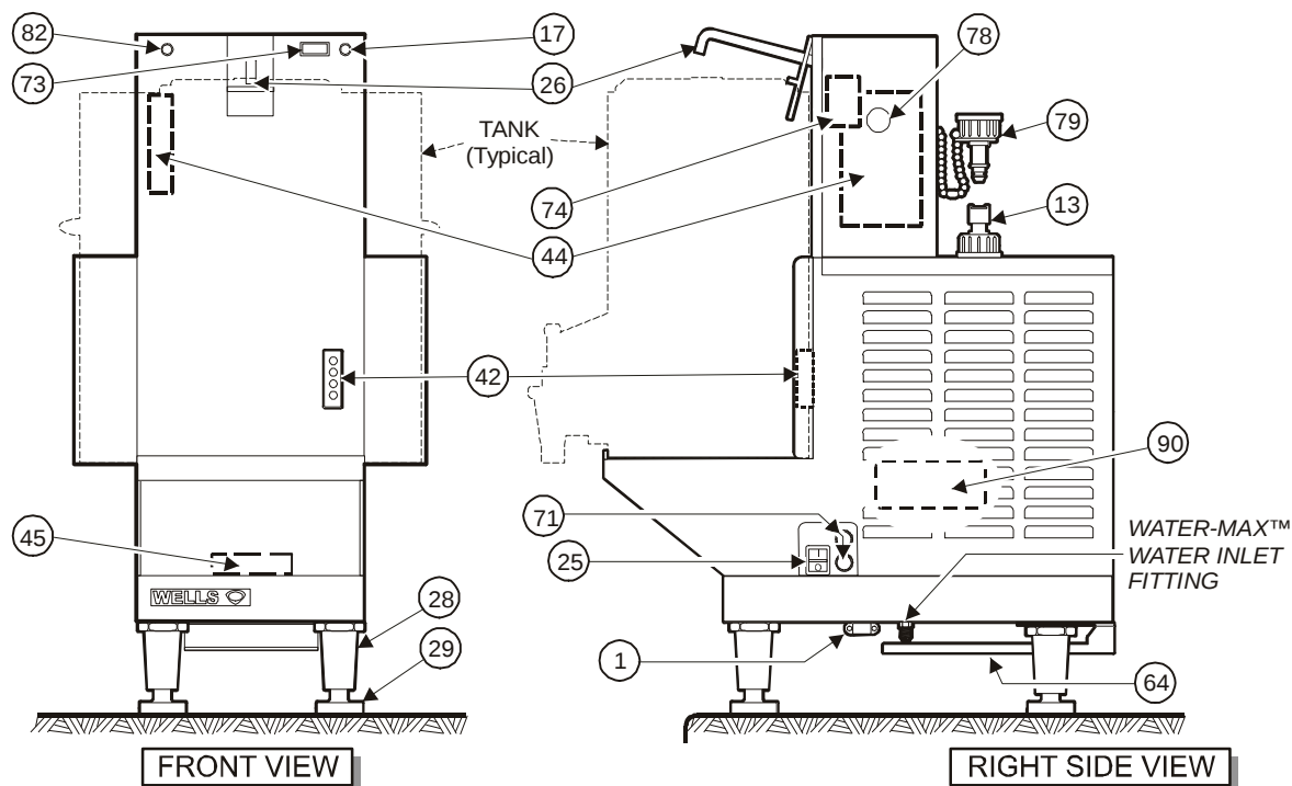
Fig. 1 Features & Operating Controls - Water Max™ Dispenser
