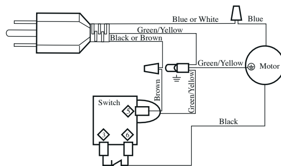
Wiring Diagram (current production)
