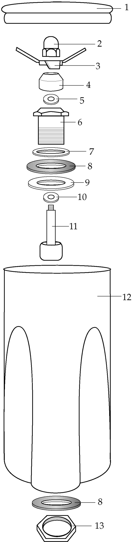
501580 Blending Assy.
