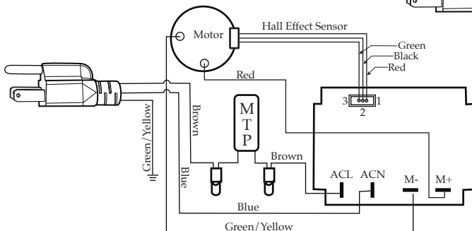
Wiring Diagram
