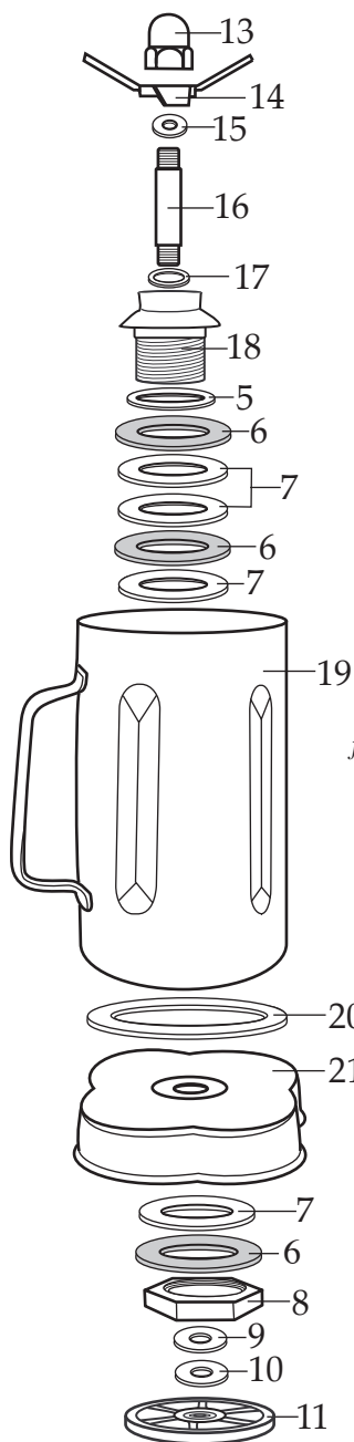
007314W Blending Assy. 500757 Container with Blending Assy. 500750 Container with Blending Assy. and Lid
