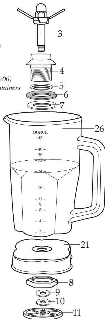
503215 - BB900M, BB900P & BC900P Container with Blending Assy. (current production)
