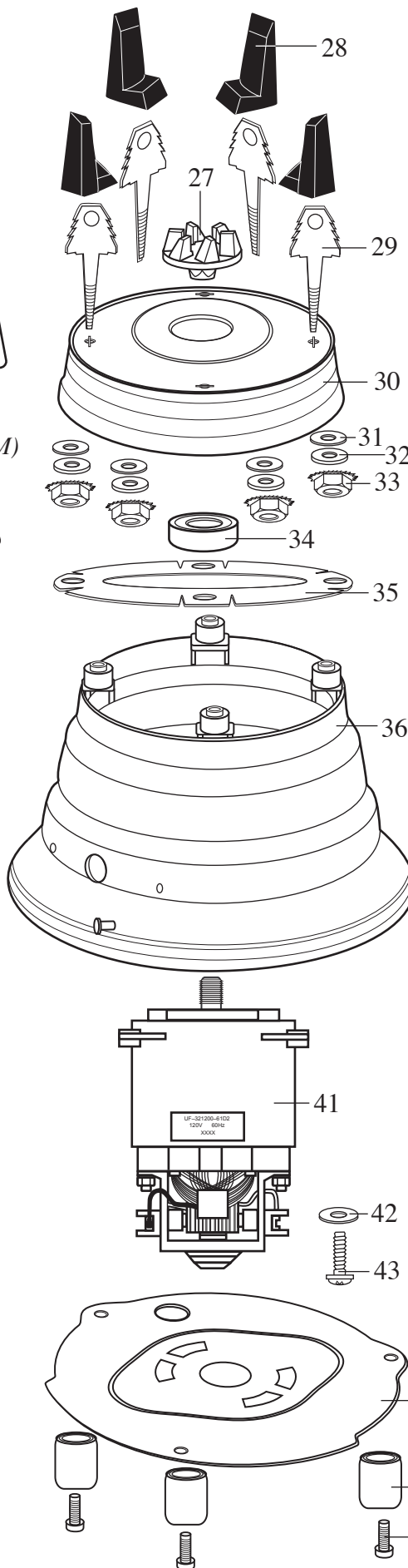
502692 Bottom Plate Assy. (metal) BC900 Units
