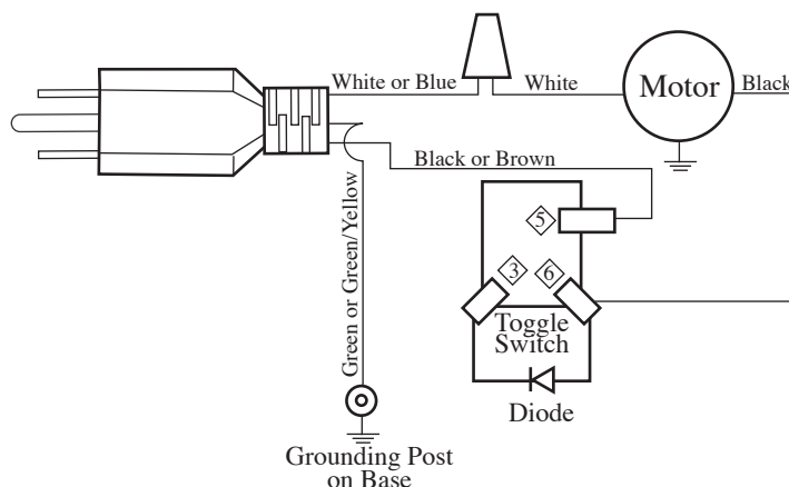
Wiring Diagram BB900G-BB900P-BB900S
