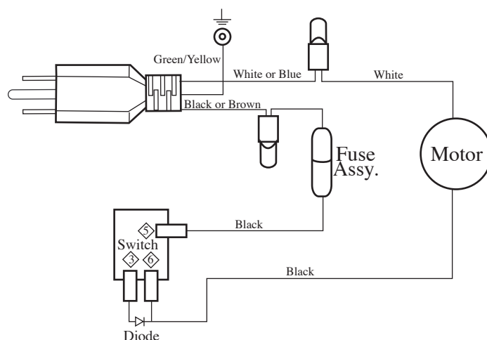
Wiring Diagram BC900G-BC900P-BC900S
