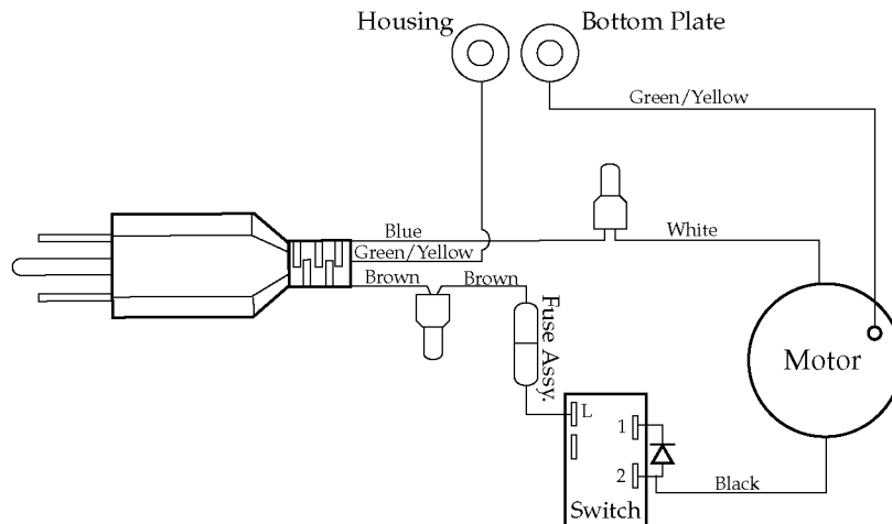
Wiring Diagram
