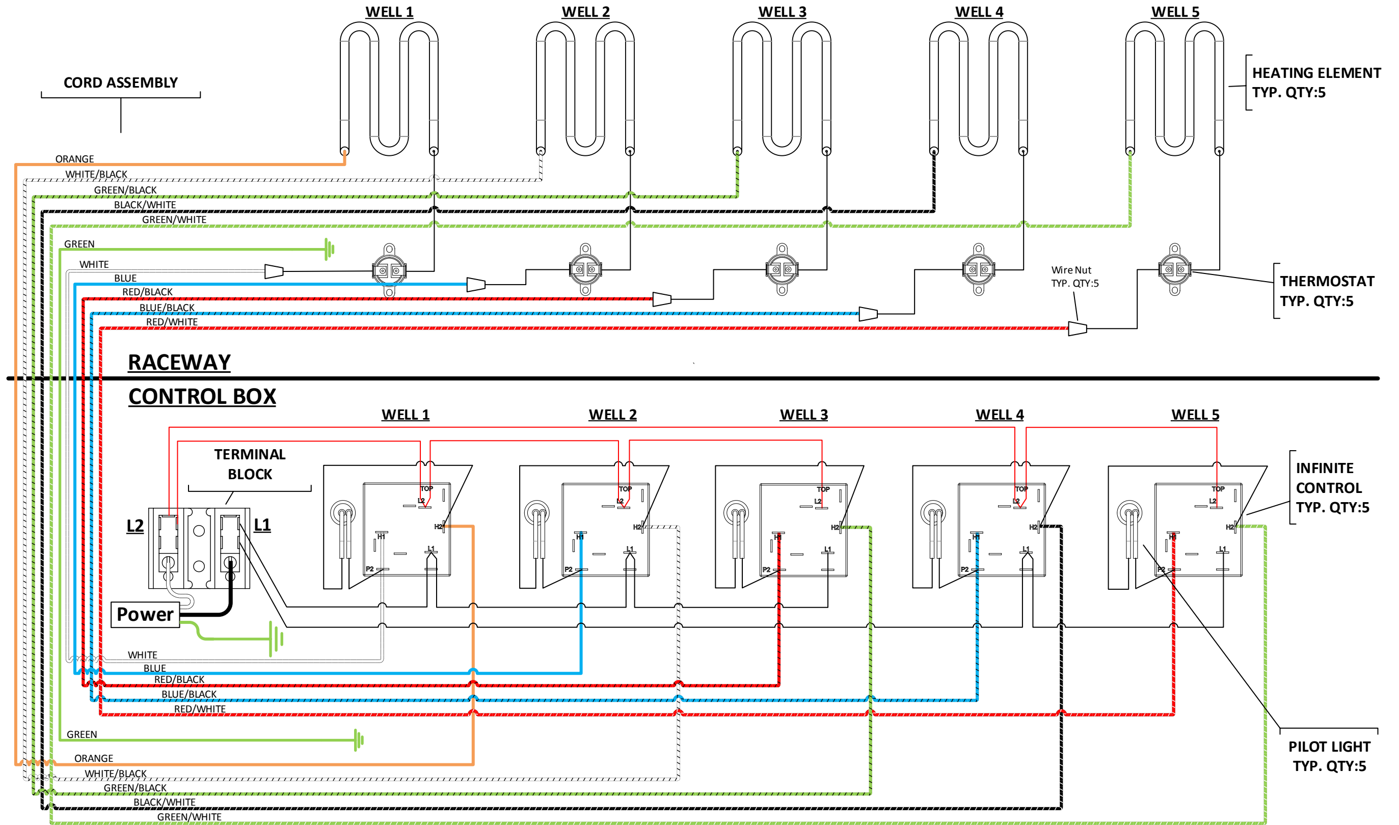
INFINITE CONTROL SCHEMATIC
