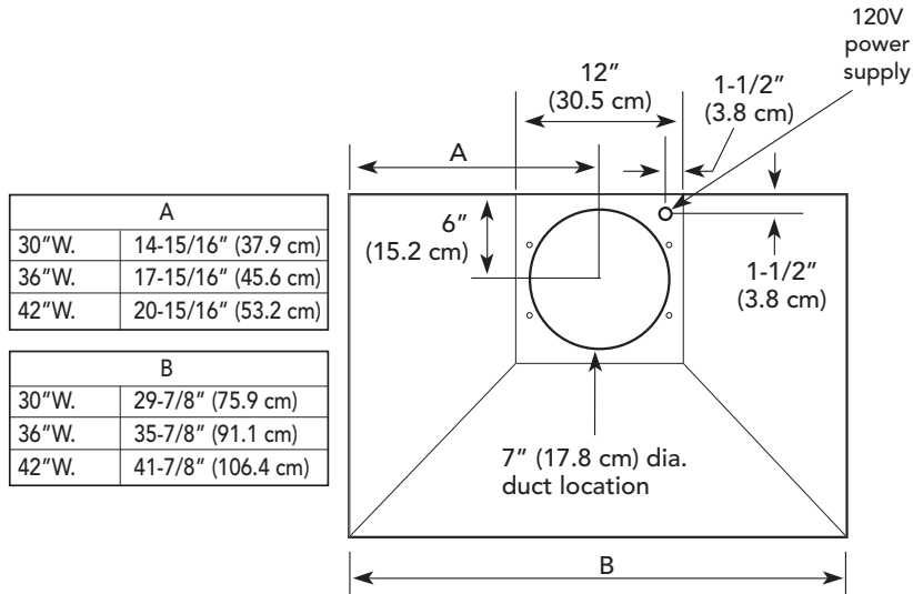
300 or 600 CFM Interior Ventilator Installation for 30", 36", & 42" models
