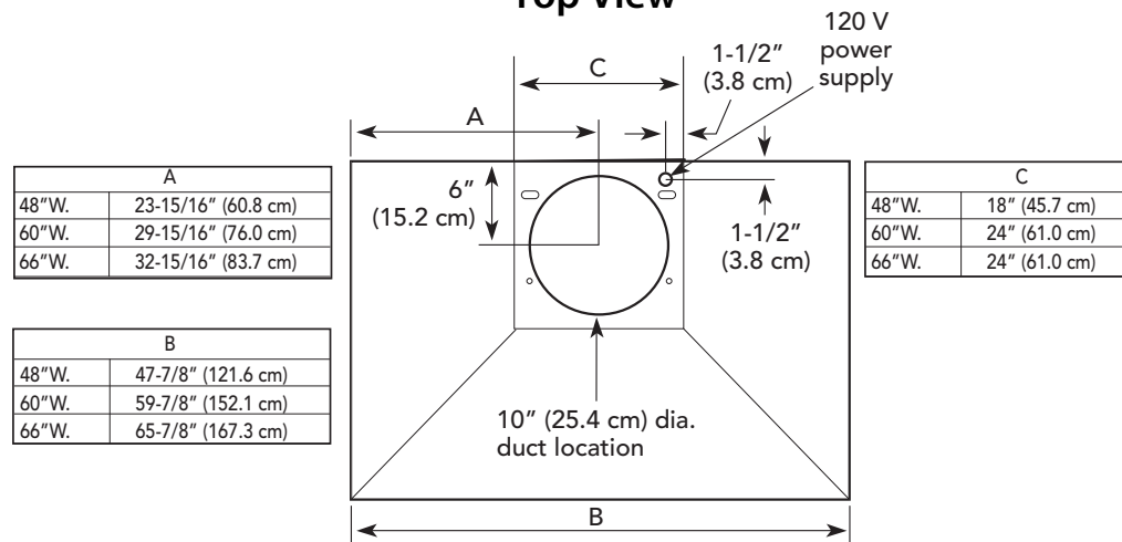
1200 CFM Interior Ventilator Installation for 48", & 60" models
