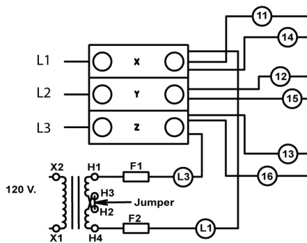
TERMINAL BLOCK WIRING FOR 480 VOLT 3 PHASE OPERATION
