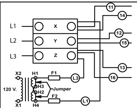
TERMINAL BLOCK WIRING FOR 208/240 VOLT 3 PHASE OPERATION (Factory Configuration)
