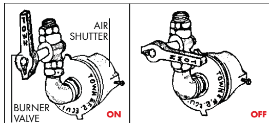
FIGURE 2 BURNER VALVE SHOWN WITH AIR SHUTTER (RING BURNERS ONLY)
