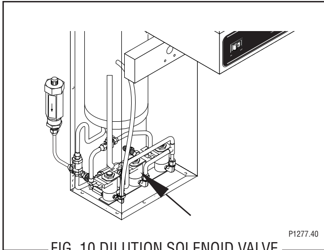
FIG. 10 DILUTION SOLENOID VALVE
