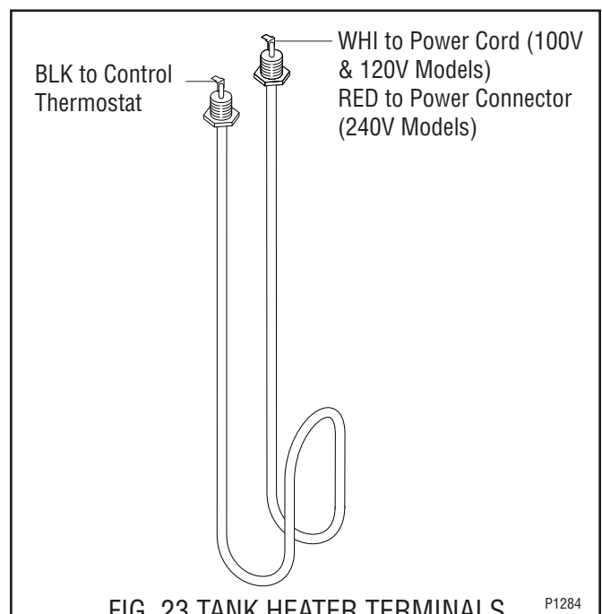
FIG. 23 TANK HEATER TERMINALS
