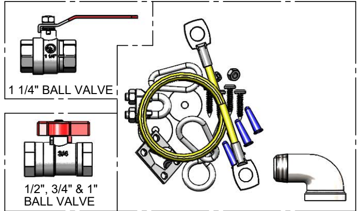
Installation Kit: Restraining Cable, Street El, Ball Valve and 90° Elbow
