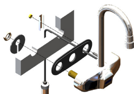
4" C/C (2D,2E)
