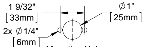
Mounting Hole Details
