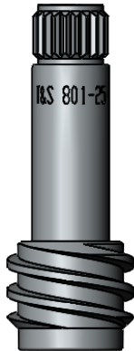
Removable Spindle, LTC (Qty = 1).
