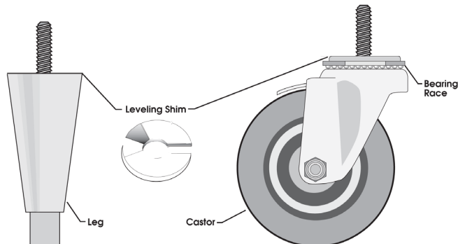
2 For leveling, insert the shim between the castor and frame rail.
