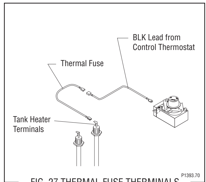
FIG. 27 THERMAL FUSE TERMINALS
