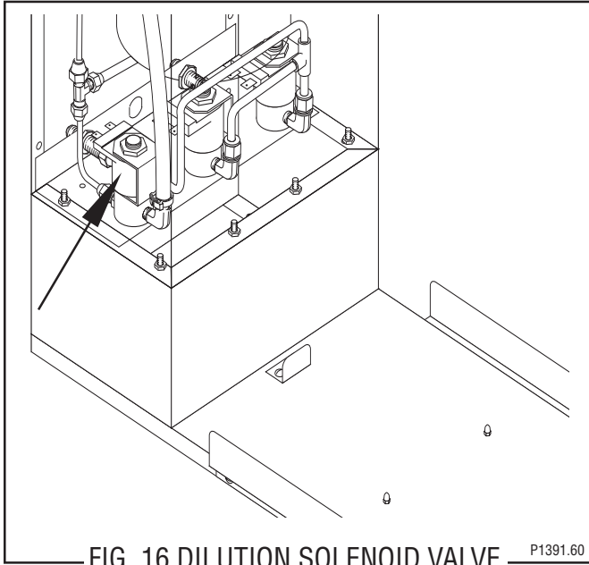
FIG. 16 DILUTION SOLENOID VALVE P1391.60
