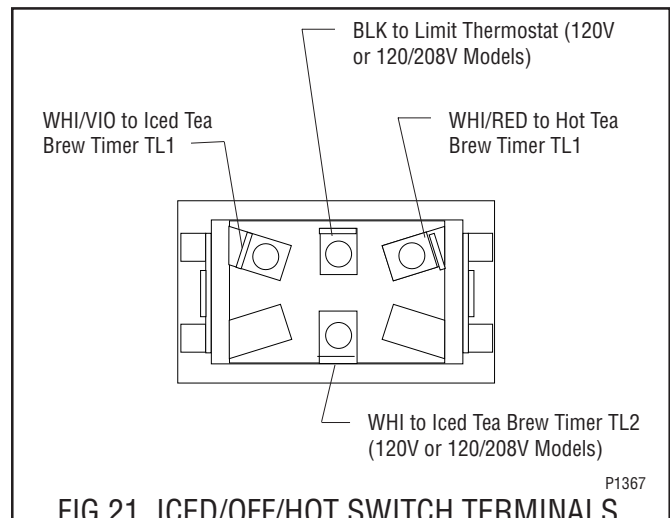
FIG. 21 ICED/OFF/HOT SWITCH TERMINALS
