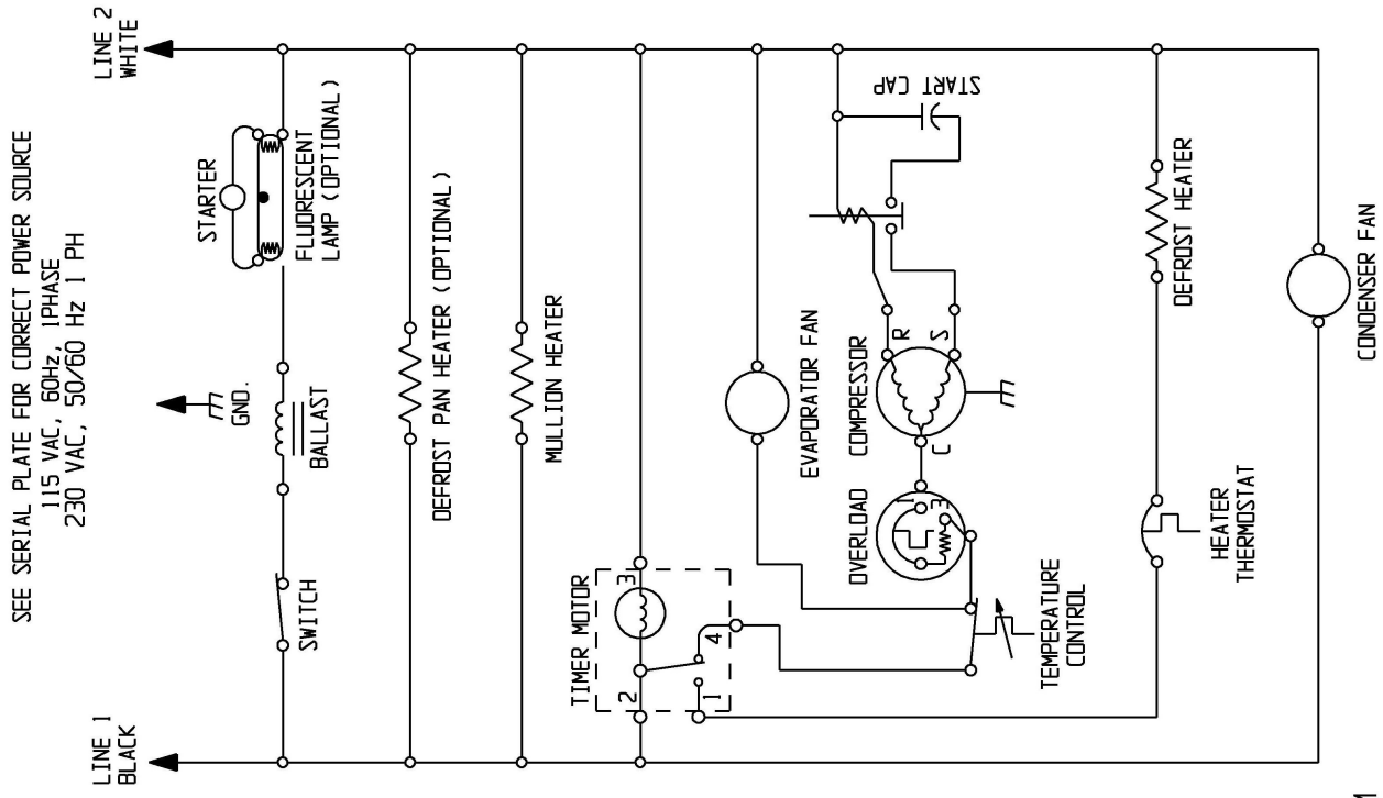
WIRING DIAGRAM MODEL SKUCF7F
