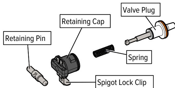
Figure 3-6 Spigot Components
