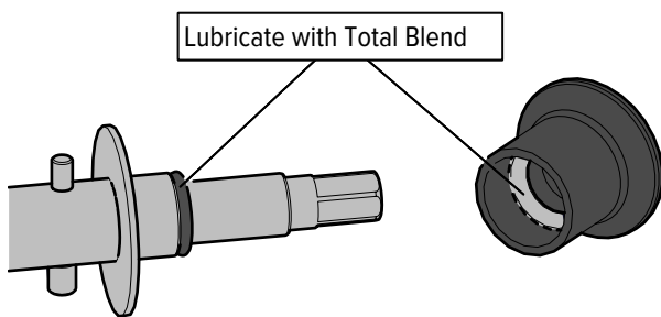
Figure 3-6 Lubricate Rear Seal
