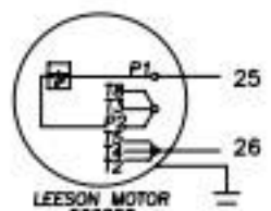
DETAIL A (115 V APPLICATION)
