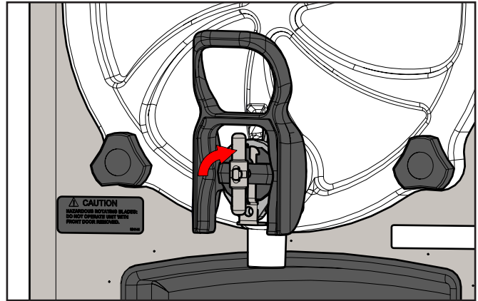
Figure 3-2 Remove Spigot Handle
