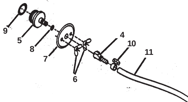
Figure 6. Manifold Disassembly
