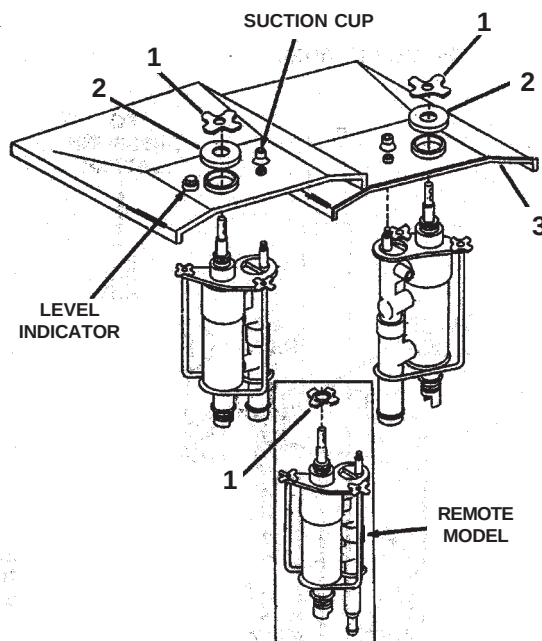
Figure 5. Pump Assembly Removal
