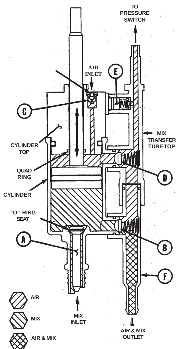
Figure 4. Pump Operation
