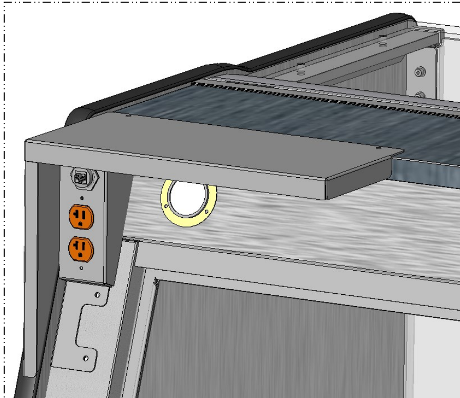
← View of Typical Case With Scale Stand, Receptacle and CAT-5 Connector
