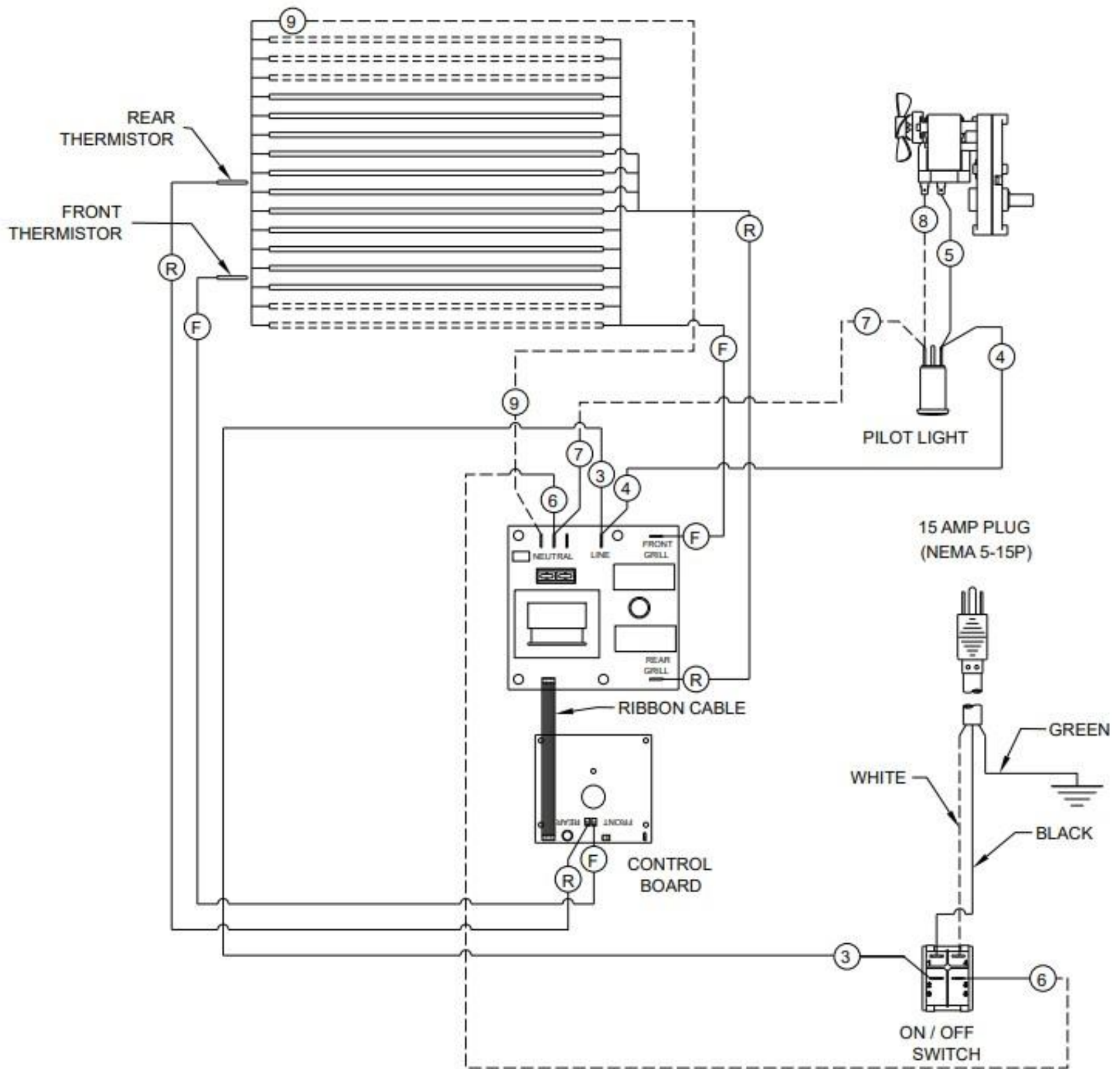
WIRE DIAGRAM, ELECTRONIC TRI-ZONE ROLLER GRILLS
