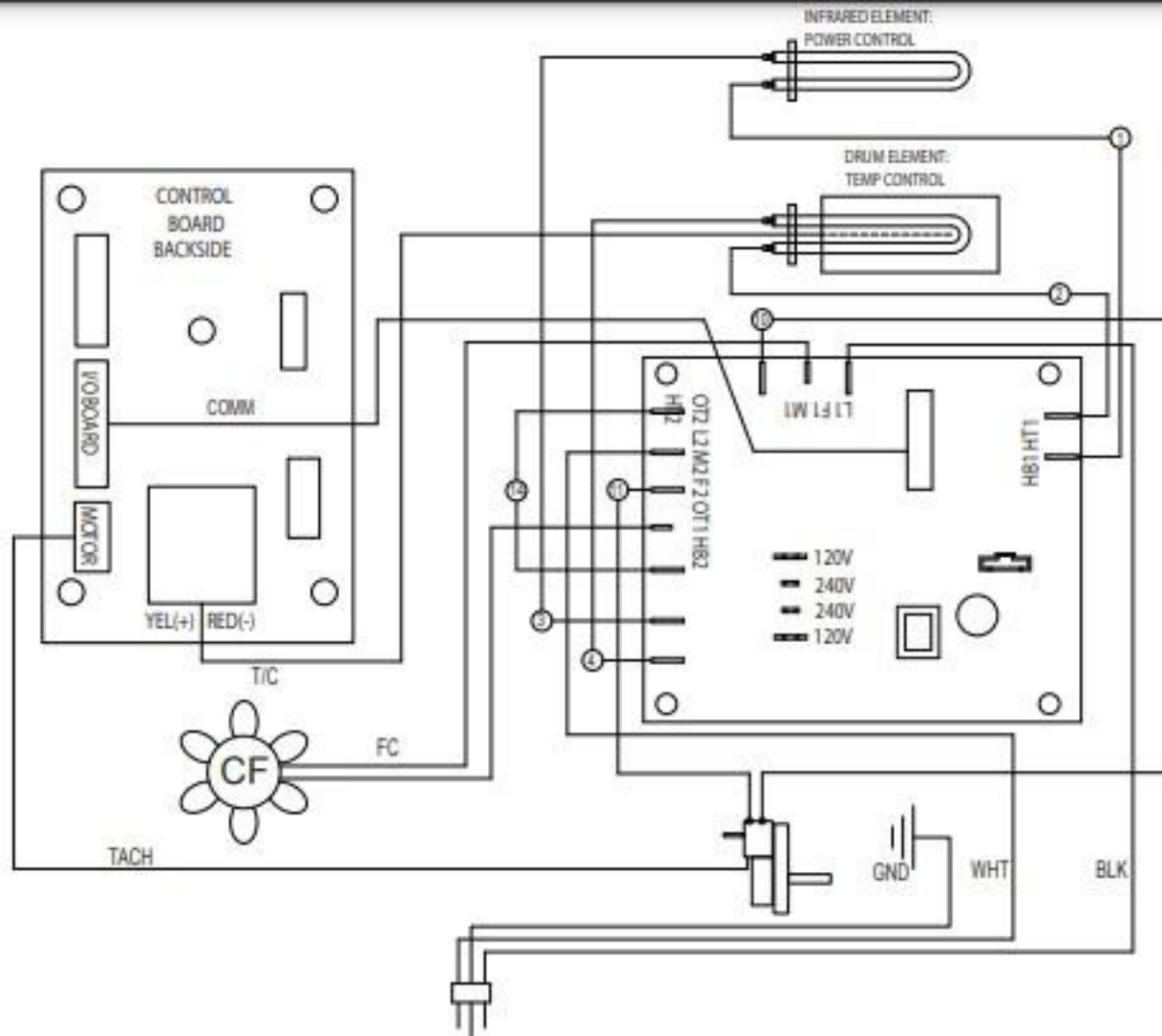
WIRING DIAGRAM RTW-E
