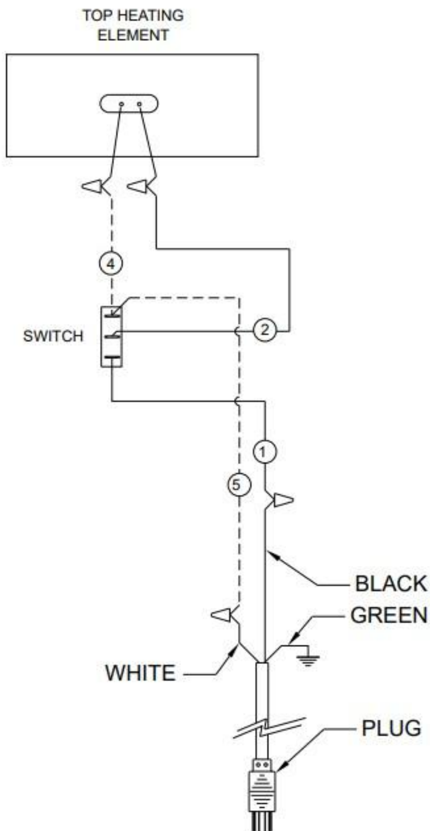
MODEL: HWP-1C WIRE DIAGRAM, 120V SK2499 03/14/11
