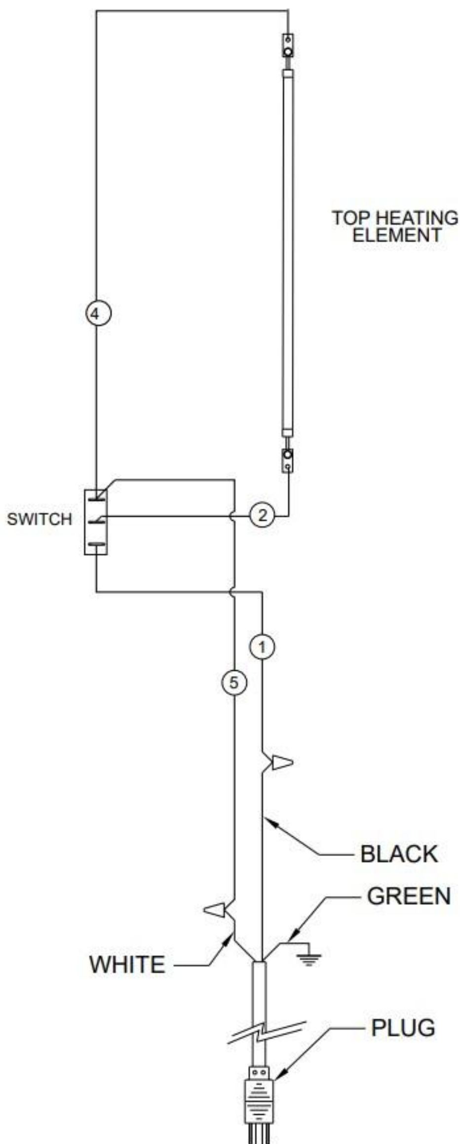
MODEL: HWP-1 WIRE DIAGRAM, 120V SK2498 03/14/11
