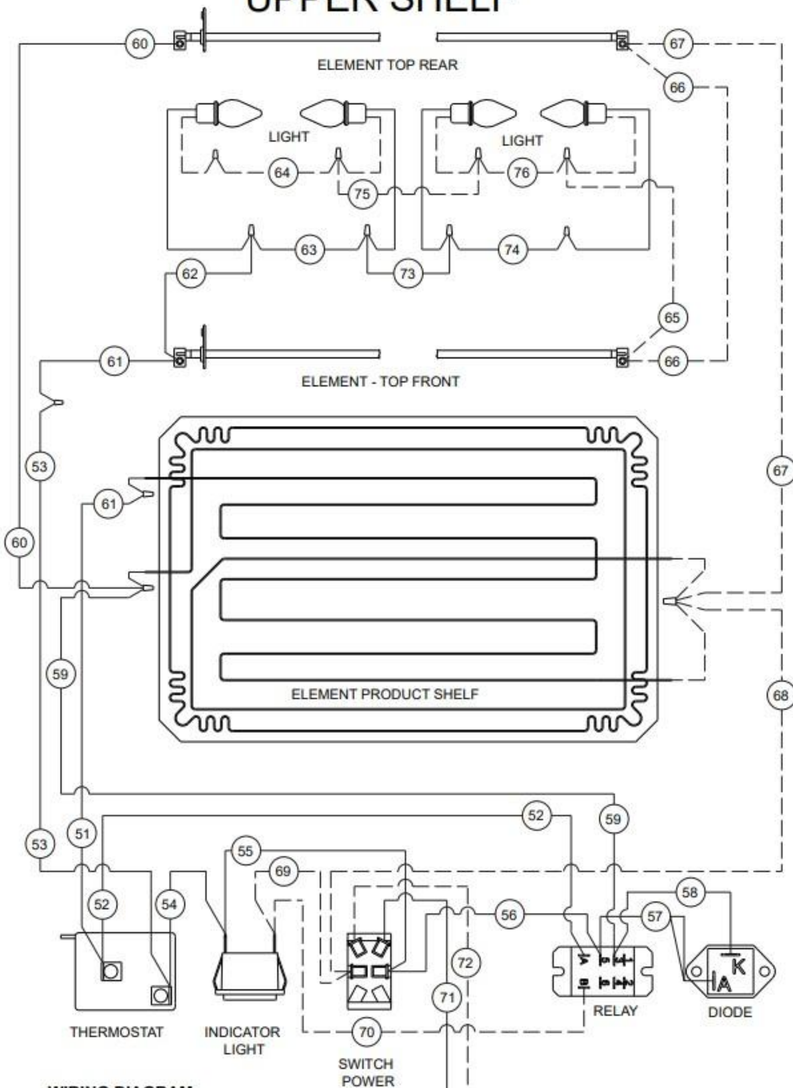
WIRING DIAGRAM. DUAL SHELF. 4 LIGHTS PER SHELF. L14-20 PLUG.
