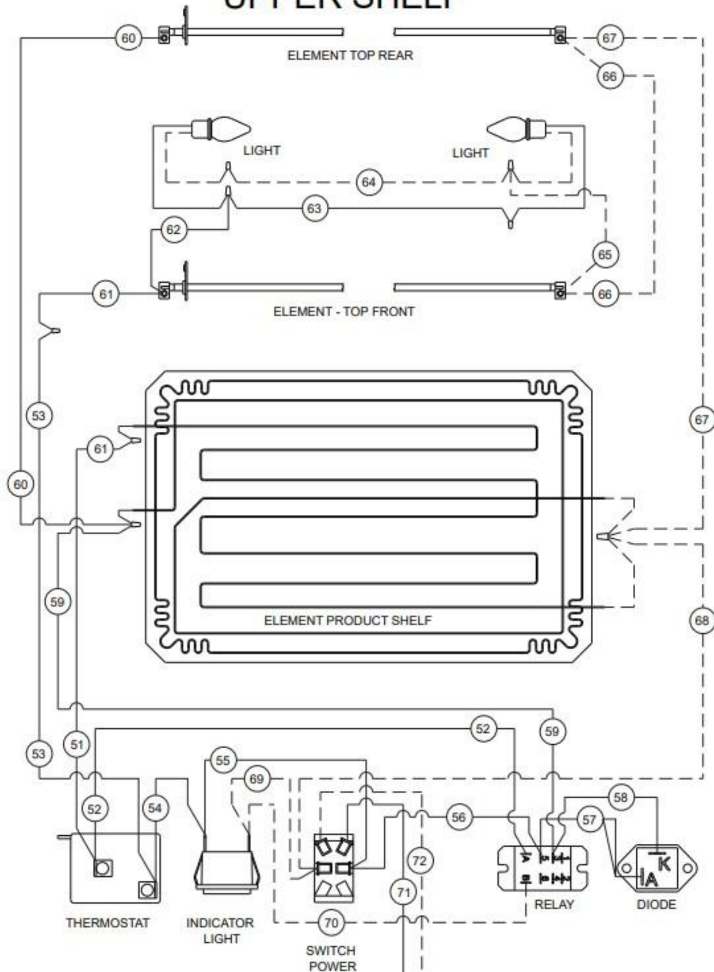
WIRING DIAGRAM. DUAL SHELF. 2 LIGHTS PER SHELF. L14-20 PLUG.
