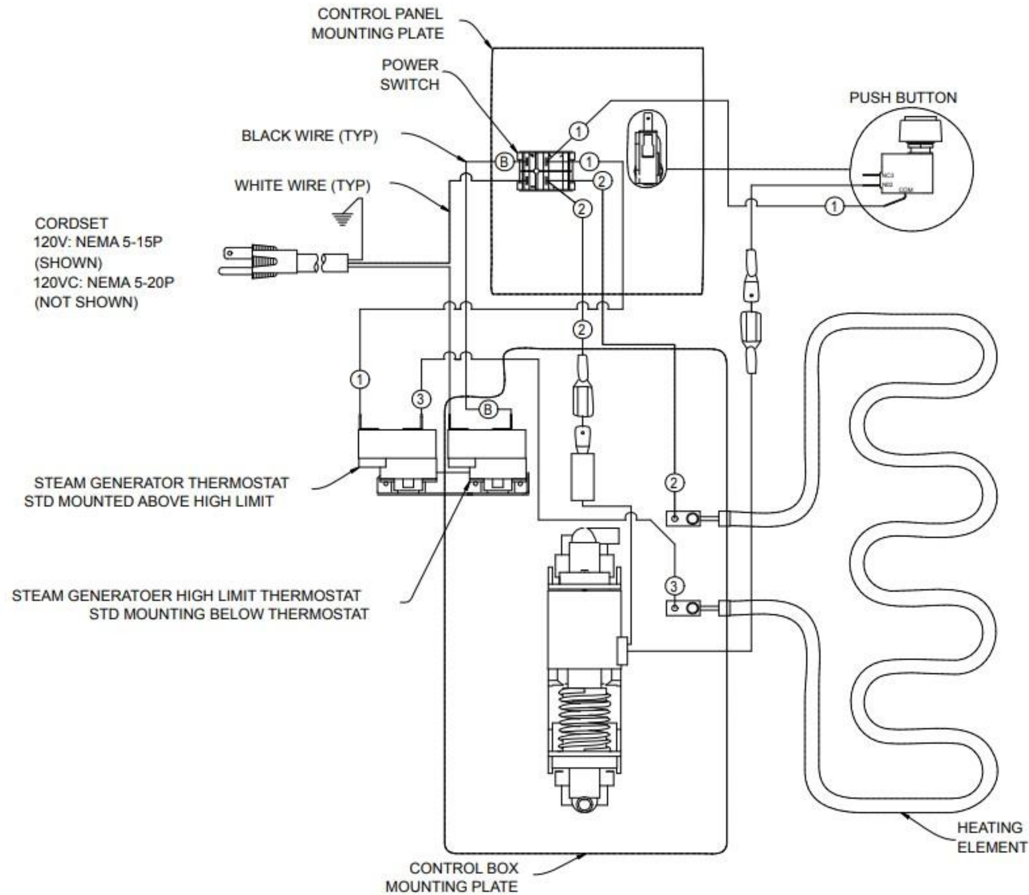
WIRING DIAGRAM FS1R & FS2R
