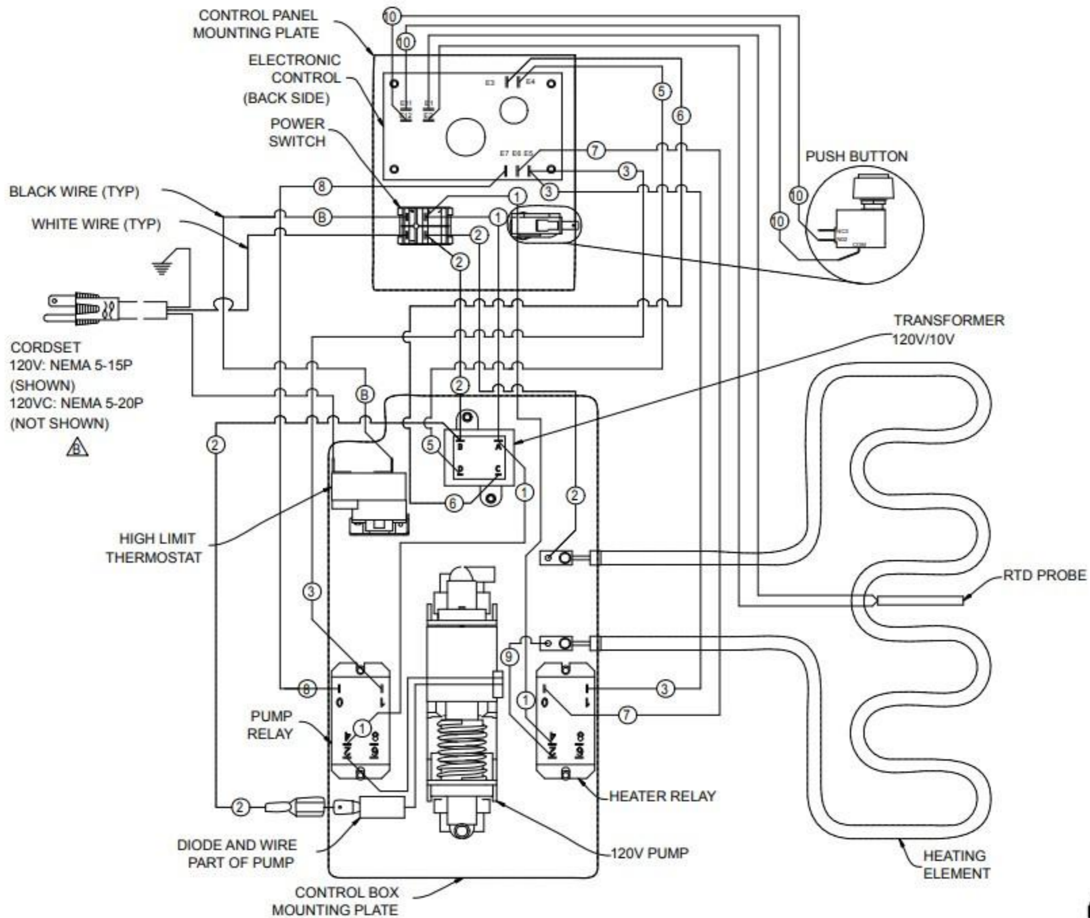
WIRING DIAGRAM FS1RT & FS2RT COMPLETE
