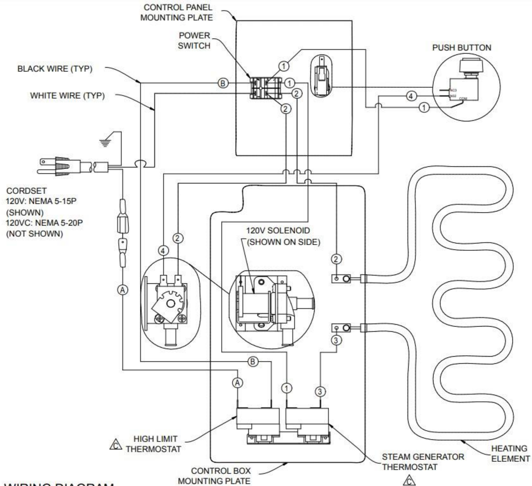
WIRING DIAGRAM FS1D & FS2D
