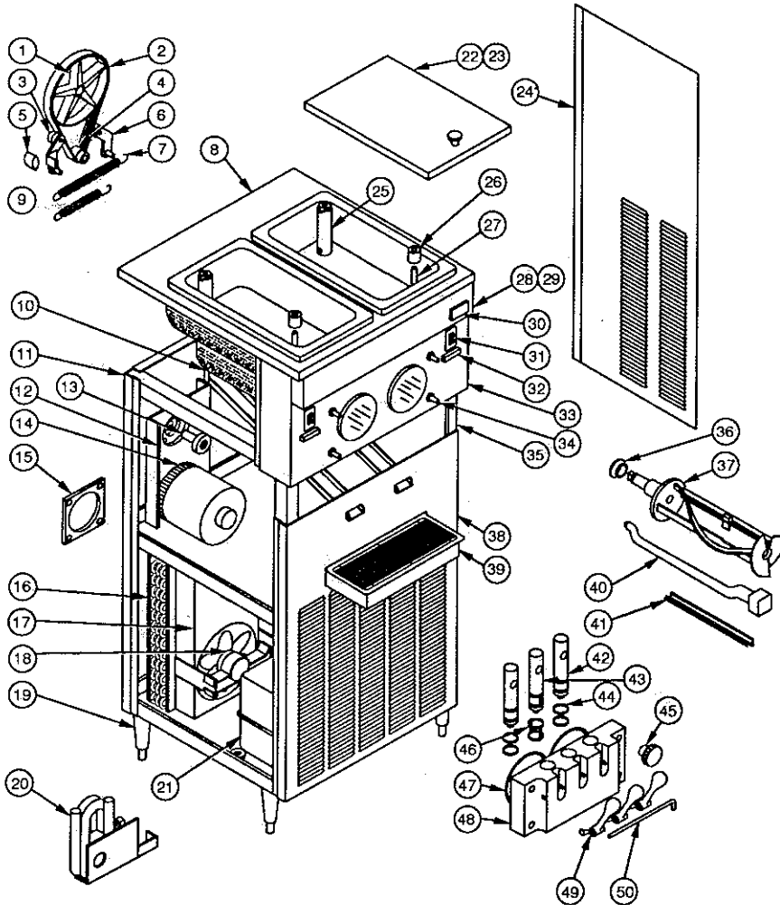
Exploded View
