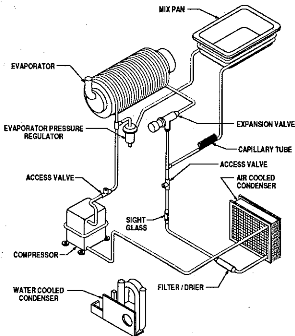
Refrigeration System
