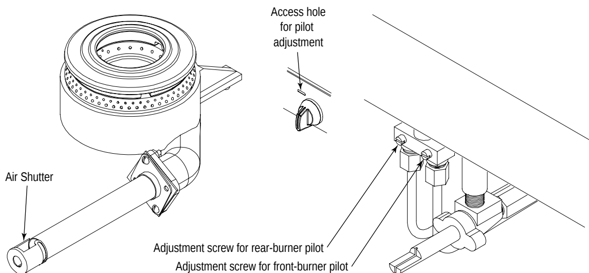
45K-Open-Burner Model
