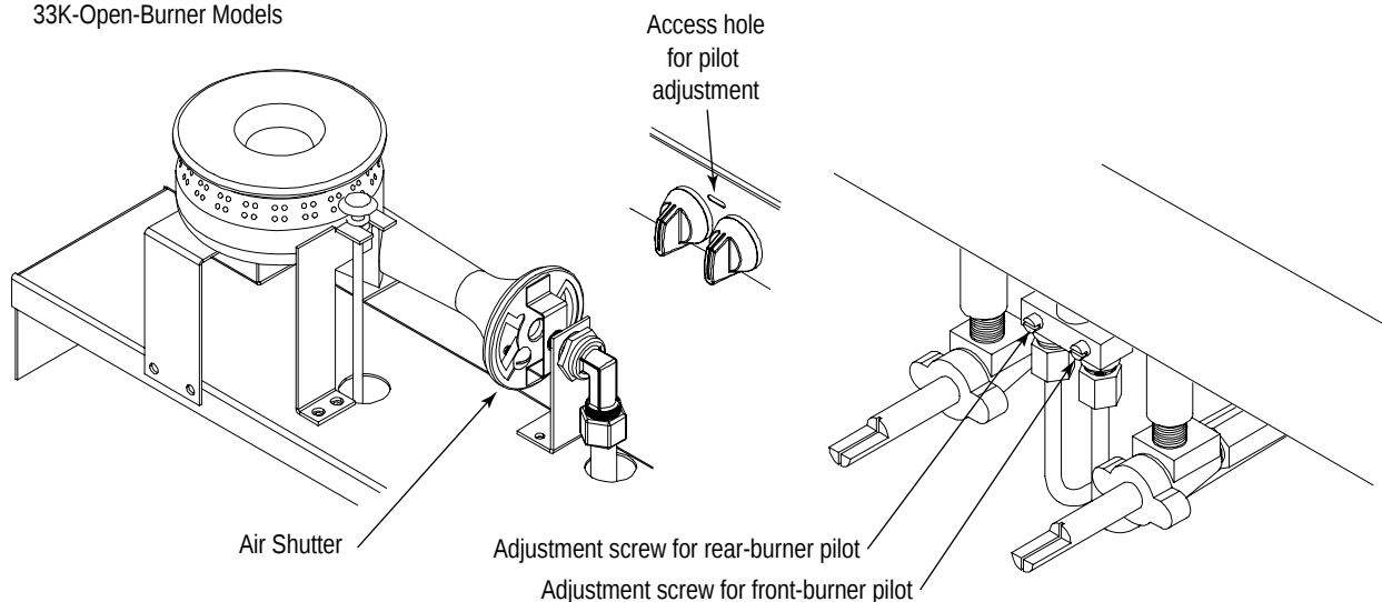
33K-Open-Burner Models
