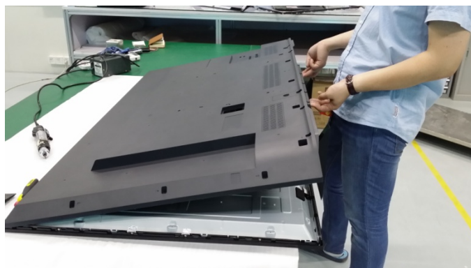
Lift up the rear cover from the bottom
