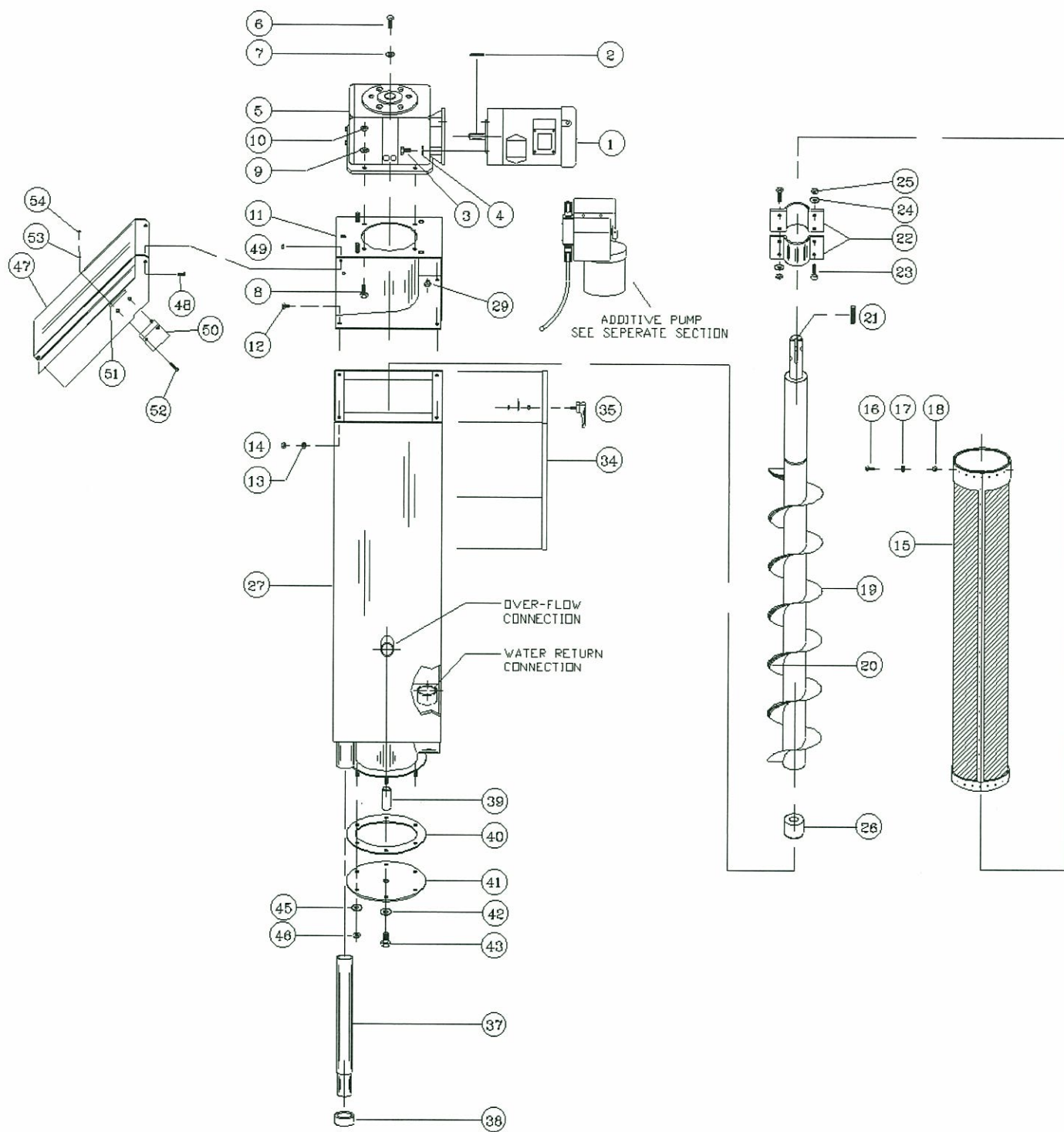
FIGURE 2. HYDRA-EXTRACTOR® HE-6CC, EXPLODED VIEW
