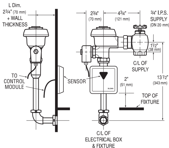
MODEL 195 ES-SM
