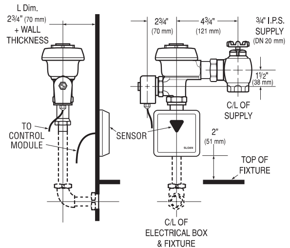
MODEL 194 ES-SM
