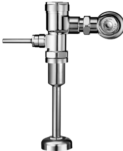
Urinal Flushometer for 1 1/4" Top Spud MODEL 180 Urinal Flushometer for 3/4" Top Spud MODEL 186
