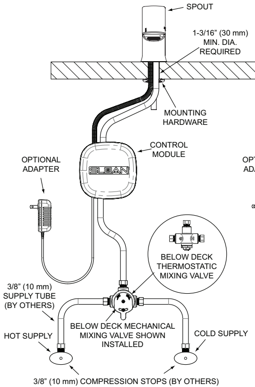
EFX-3X0.X1X.0000 WITH HOT/COLD WATER SUPPLY
