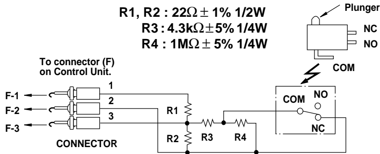
Sensor Dummy Resistor Circuit
