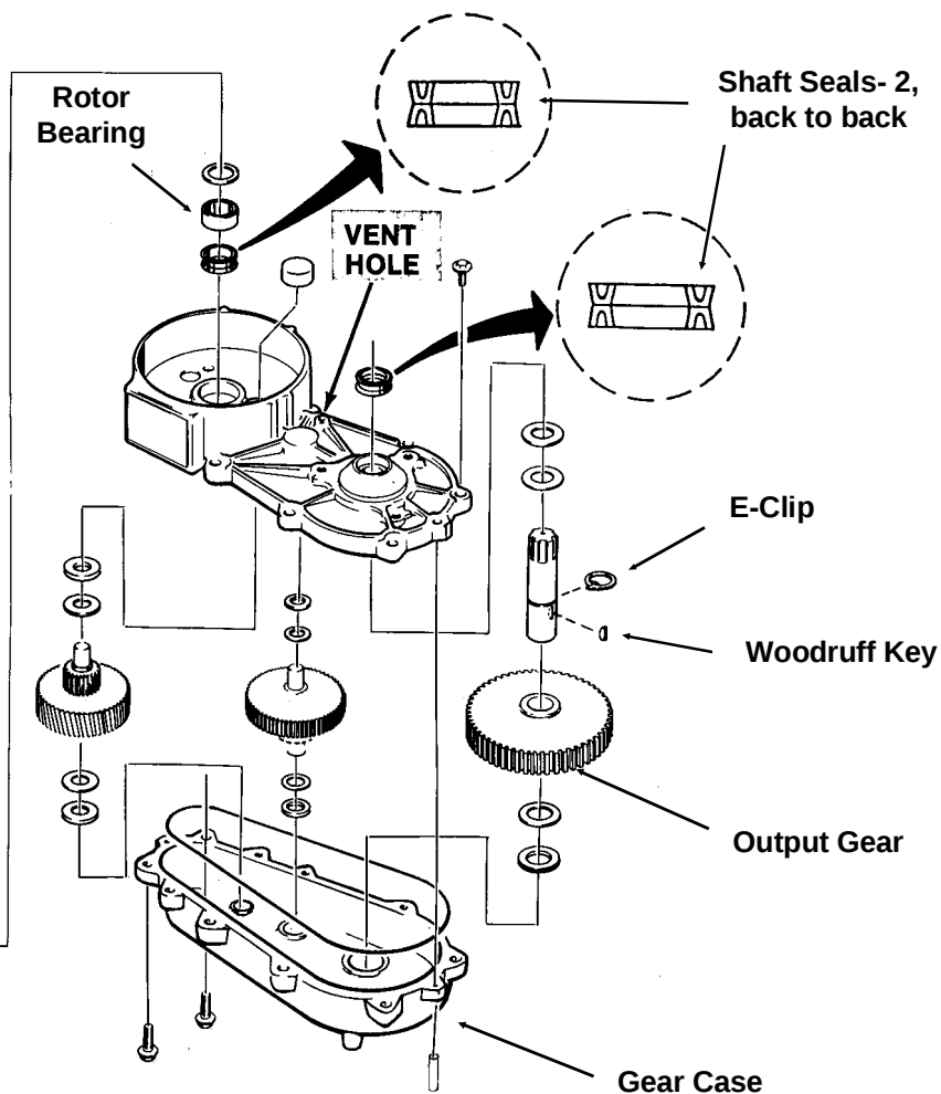
Gear Reducer Components
