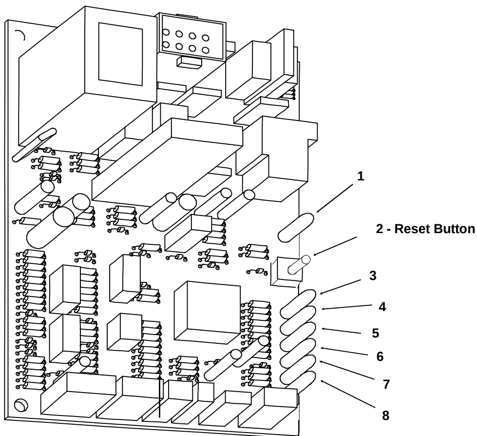
Circuit Board Light Identification
