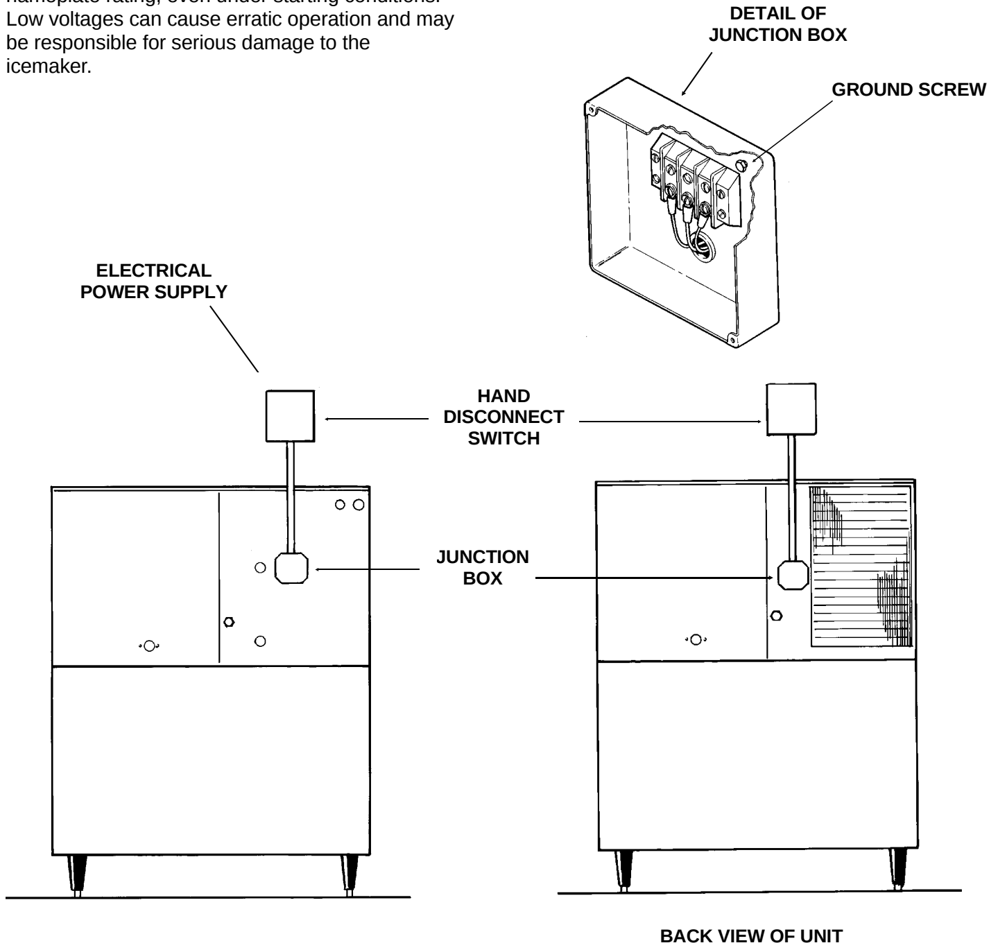
ELECTRICAL CONNECTIONS, AIR COOLED
