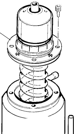
DIVIDER AND AUGER ASSEMBLY
