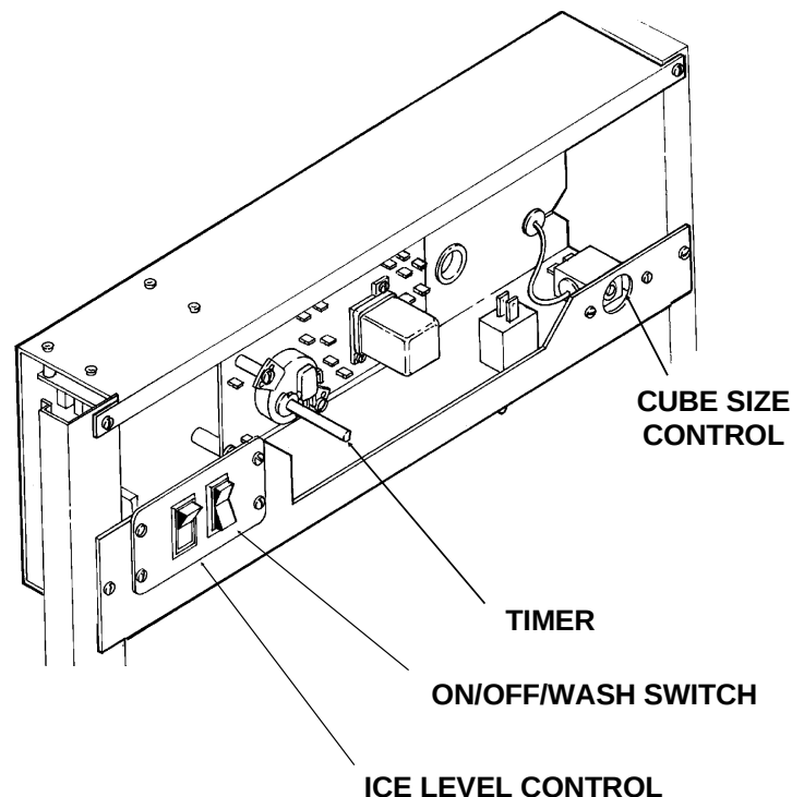
CONTROL BOX
