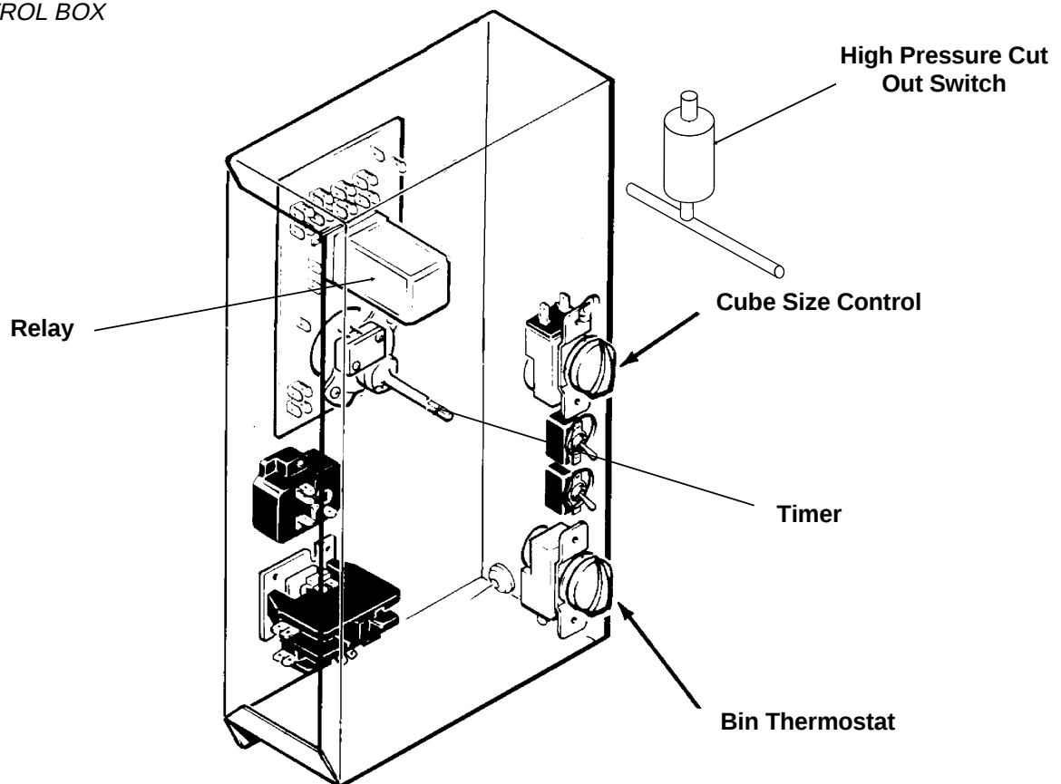
CONTROL BOX
