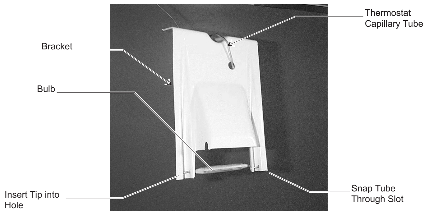
Attach Thermostat Bulb to Bracket
