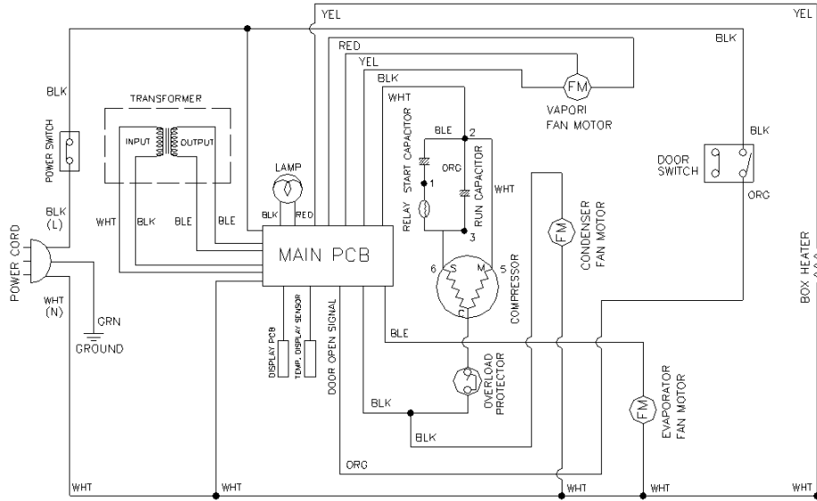
CIRCUIT DIAGRAM (T23R)
