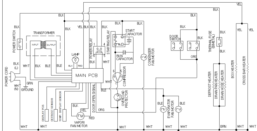
CIRCUIT DIAGRAM (T49F)
