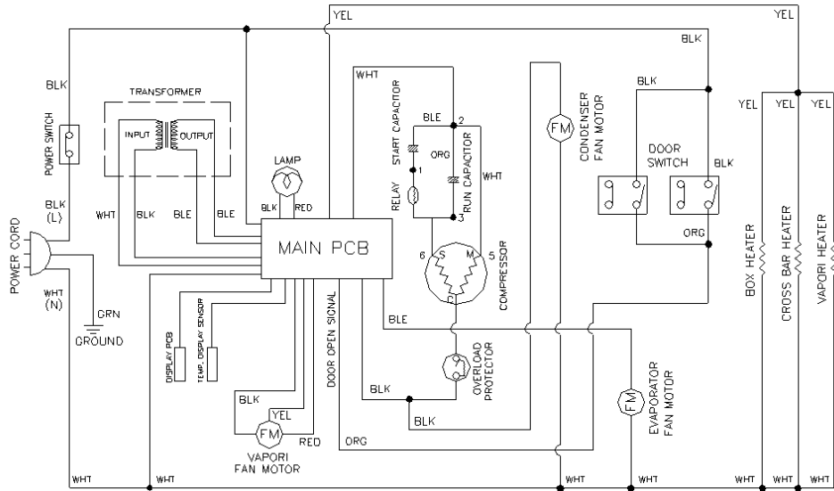
CIRCUIT DIAGRAM (T49R)
