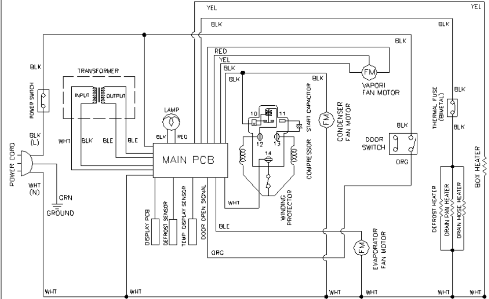
CIRCUIT DIAGRAM (T23F)
