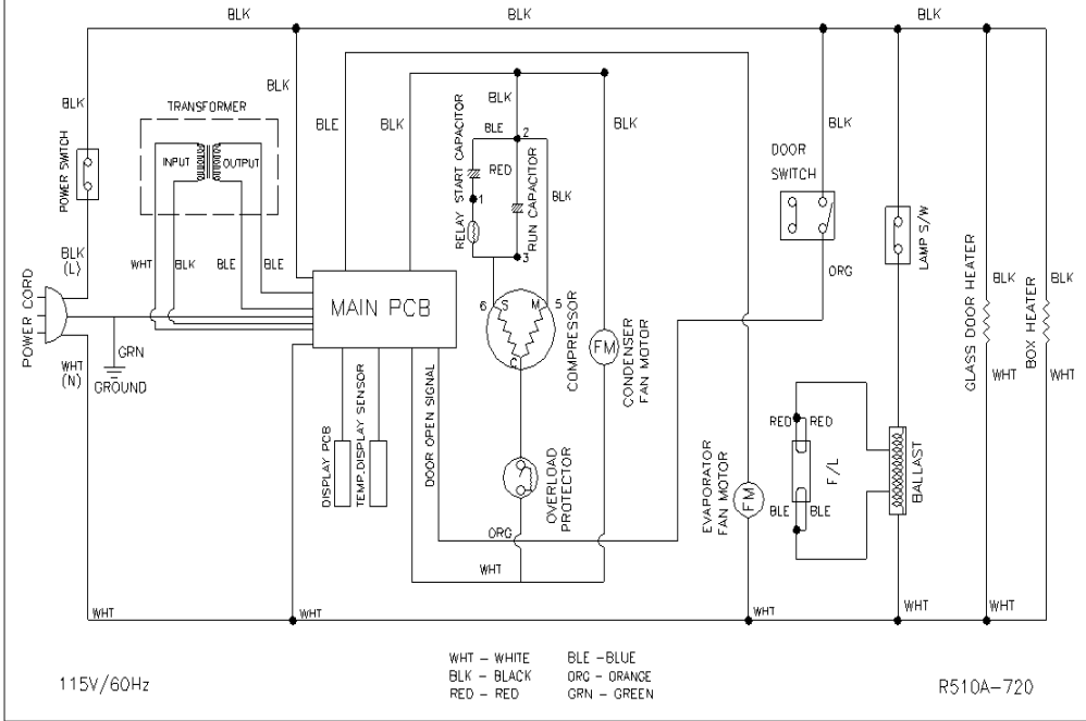
CIRCUIT DIAGRAM (B23G)
