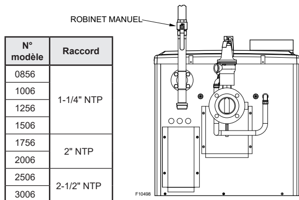
Figure 31. Raccordement du gaz
