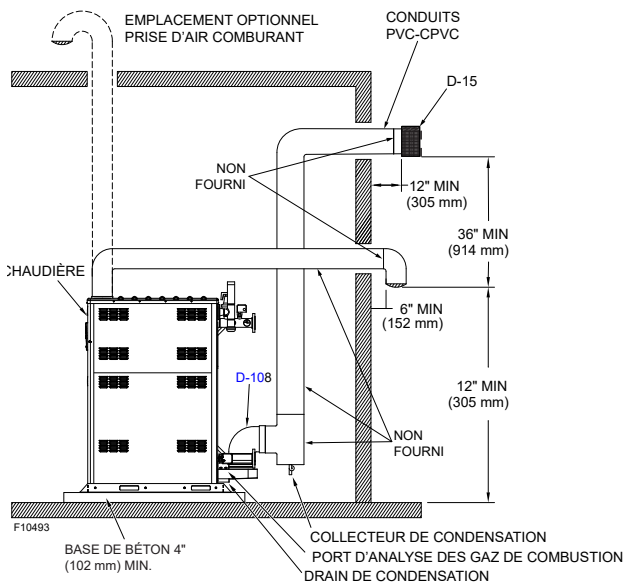
Figure 54. PVC/CPVC - Ventilation directe horizontale
