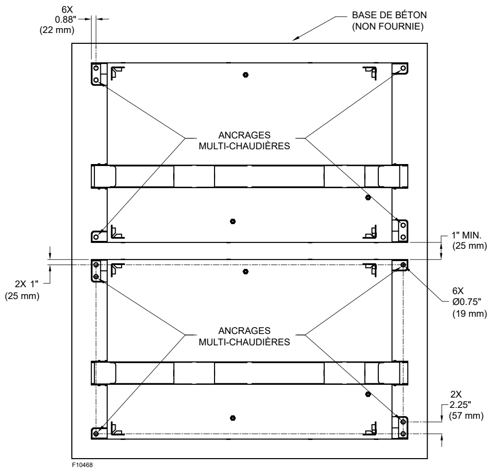
Figure 6. Ancrage multi-appareils
