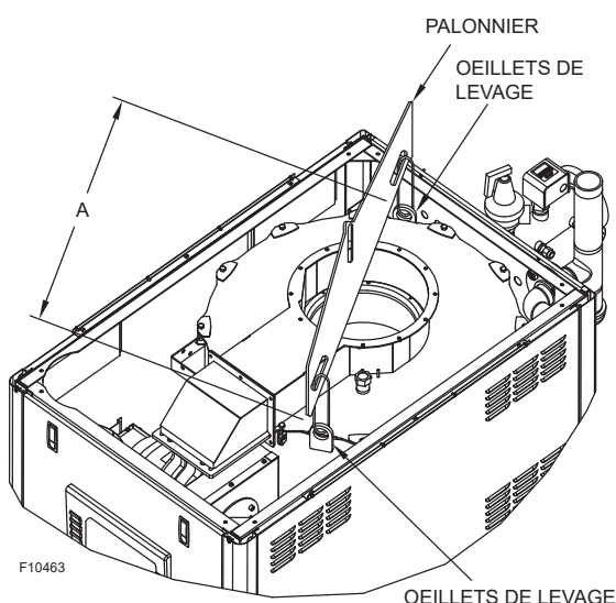
Figure 8. Oeillets de levage
