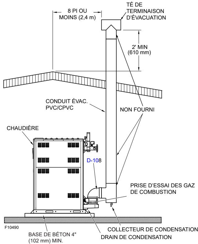
Figure 51. PVC/CPVC - Ventilation verticale
