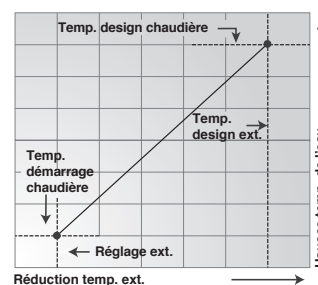
Figure 72. Ratio de compensation
