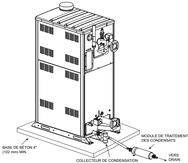
Figure 57. Illustration de la condensation
