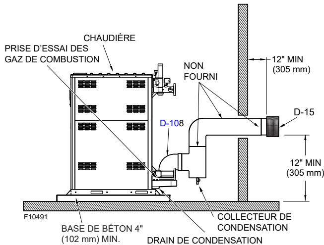
Figure 53. PVC/CPVC - Ventilation murale et horizontale
