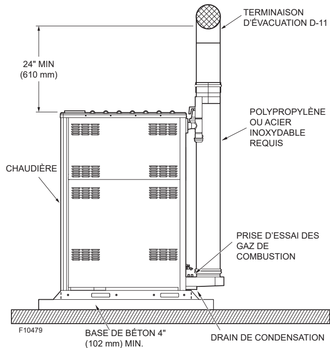
Figure 55. Installation extérieure
