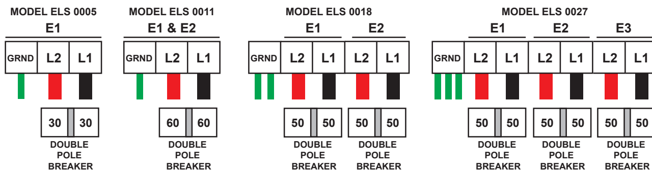
Figure 2. Wire Connection to Circuit Breakers
